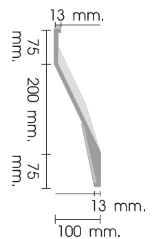
WMI 100-406
