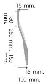
WMI 100-610
