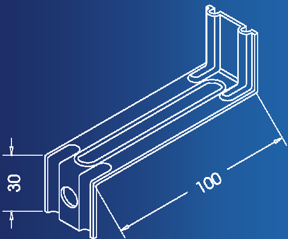
CONNECTOR LOUVER
