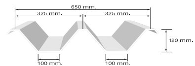
WMI 110-650BL
