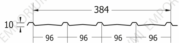
TYPE 5M
