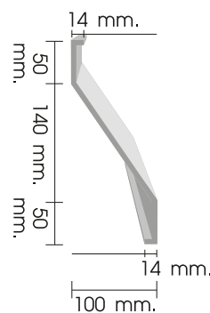
WMI 100-304
