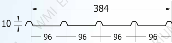
TYPE 5
